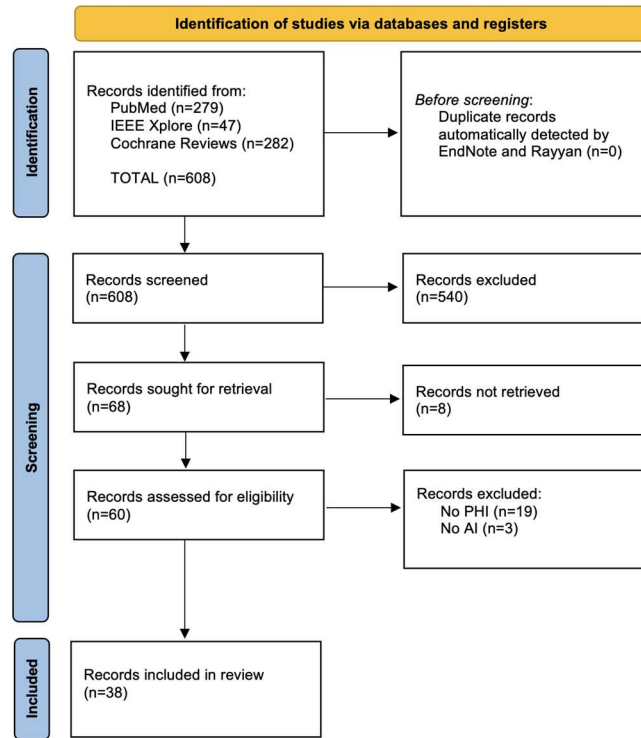
Figure 1. PRISMA flowchart
